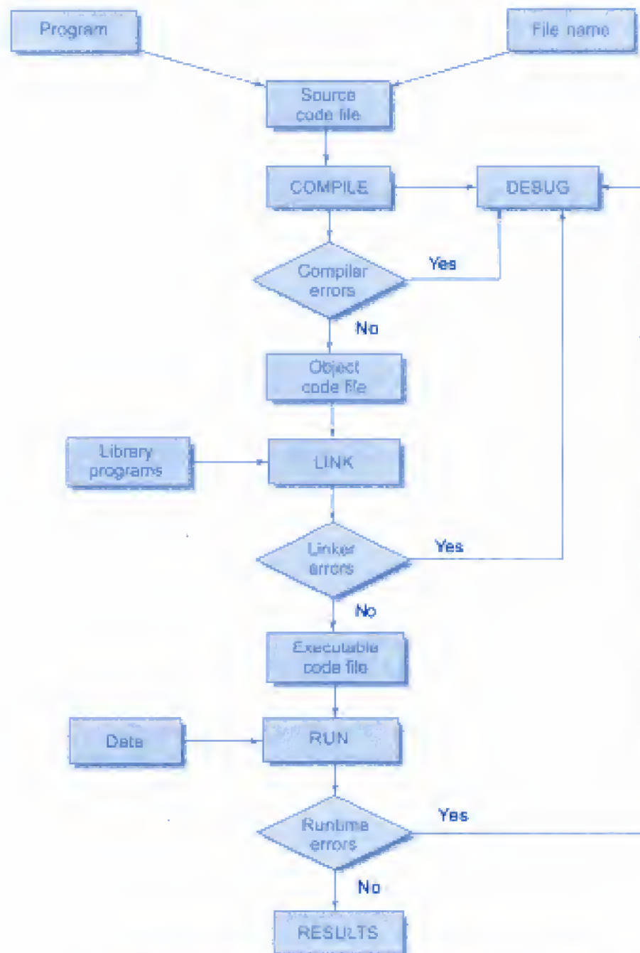
Fig. R.1 ⇔ Program development and execution
