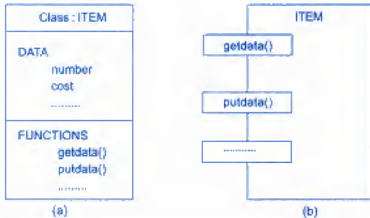
Fig. 5.2 Representation of a class
