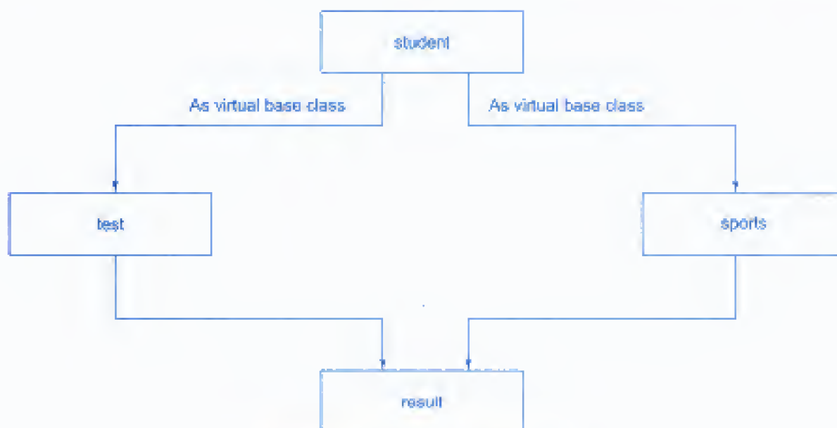
Fig. 8.13 ⇔ Virtual base class
