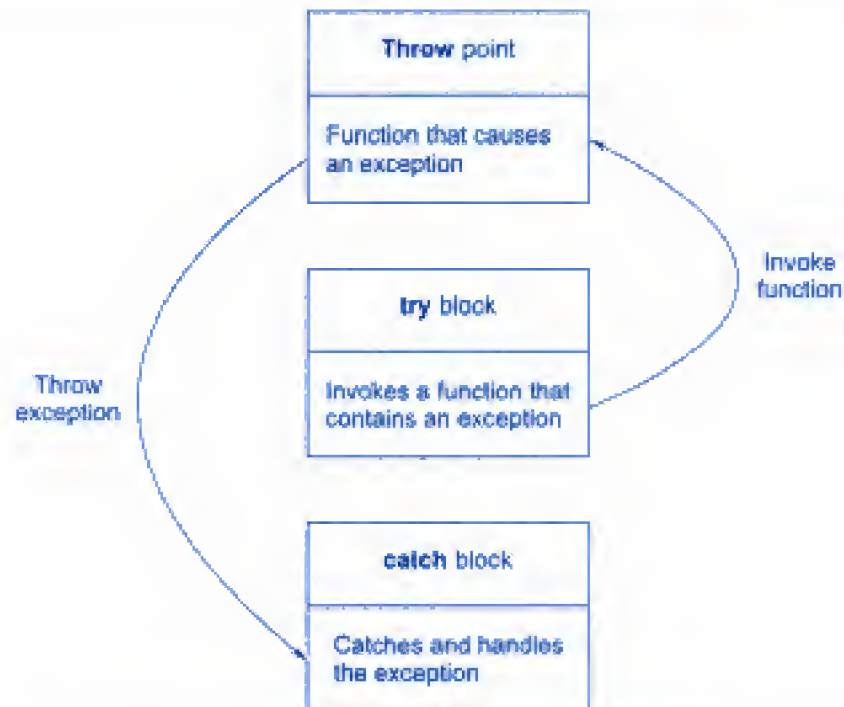
Fig. 13.2 \Leftrightarrow Function invoked by try block throwing exception
