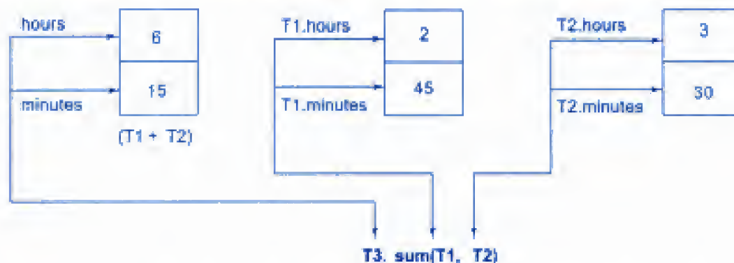
Fig. 5.6 ⇔ Accessing members of objects within a called function
