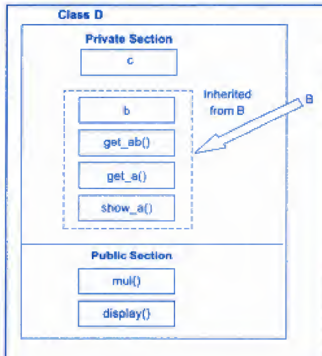
Fig. 8.3 \leftrightarrow Adding more members to a class (by private derivation)
