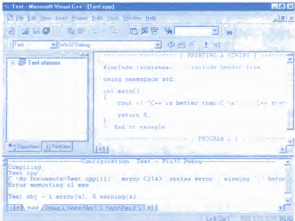
Fig. C.10 ⇔ Output window error messages
