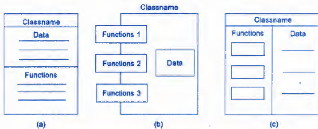
Fig. 17.6 \Leftrightarrow Various forms of representation of classes/objects
