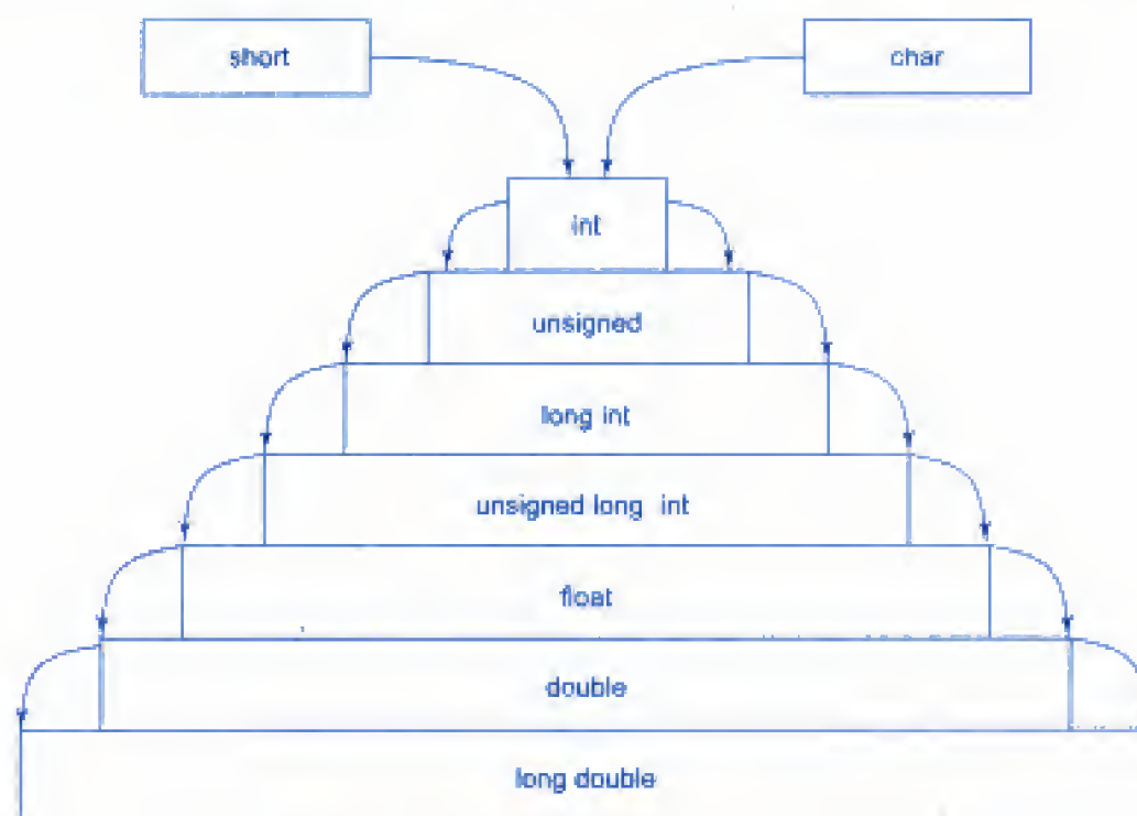
Fig. 3.3 Water-fall model of type conversion
