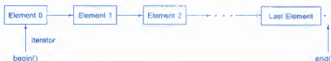
Fig. 14.3 Elements in a sequence container
