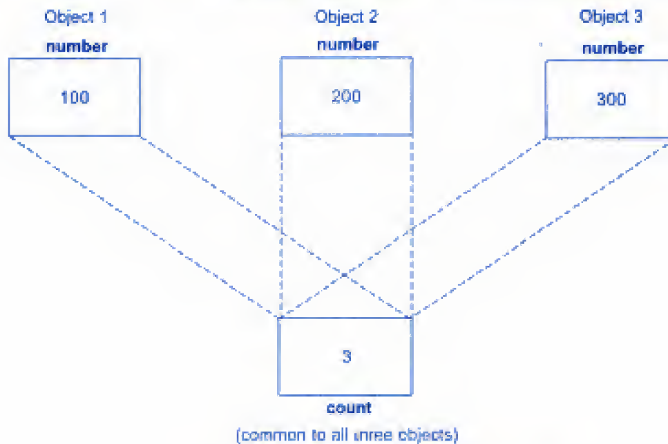
Fig. 5.4 \Leftrightarrow Sharing of a static data member
